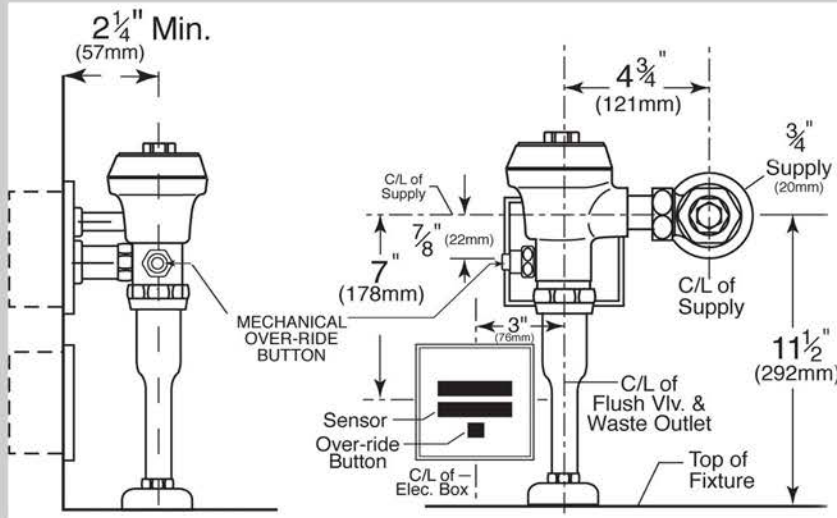
U1851 Urinal
