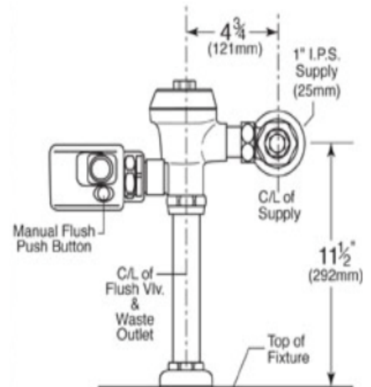
Patented TruStop Control Stop
